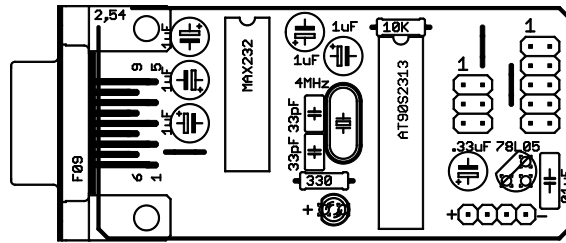
Engram Enterprises AVR910 In-System Programmer http://reboots.g-cipher.net/
